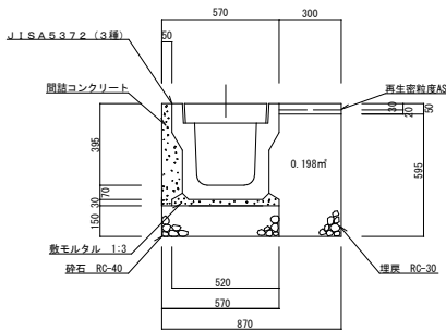
側溝300A
